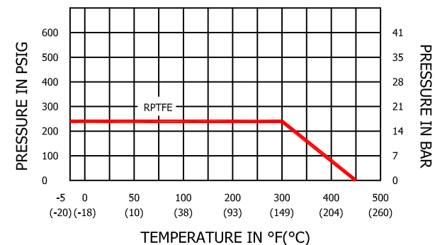
Pressure VS. Temperature Chart
